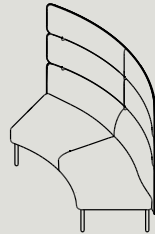
AHB60-D W 1660 D 1315 H 1350 S 440 IN Ø2400 / OUT Ø3,860
