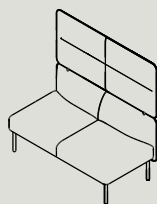
AHB2-S# W 1360 D 730 H 1350 S 440
