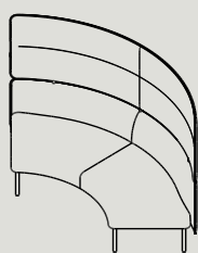
AHB90-S W 1530 D 1530 H 1350 S 440 IN Ø1600 / OUT Ø3,040
