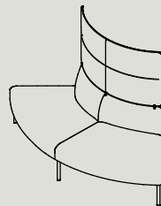
AHB90-R-S W 1480 D 1480 H 1350 S 440 IN Ø1500 / OUT Ø2,960
