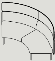
AMB90 W 1530 D 1530 H 1025 S 440 IN Ø1600 / OUT Ø3,040
