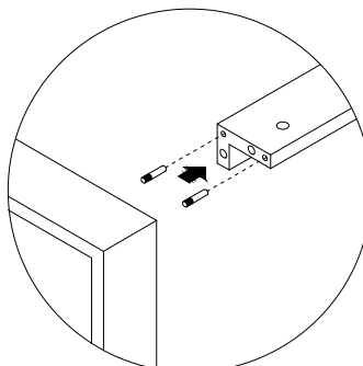
Grano Grub screw 4MA x 3
