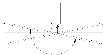
MIRROR WITH FLAT DISC B
