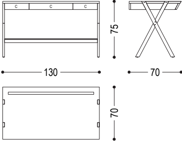
4.07.3 WITHOUT UPSTAND, 3 DRAWERS UNDER THE TOP
