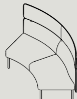
AMB60 W 1660 D 1315 H 1025 S 440 IN Ø2400 / OUT Ø3860 W 65.4" D 51.8" H 40.4" S17.3" IN Ø94.5" / OUT Ø152.0"
