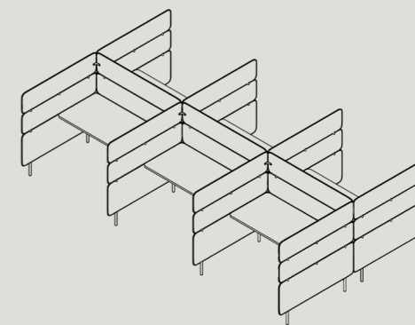
AWH-D-SPL6-B-XXXX 1330 - W 4250 / D 2845 / H 1350 1520 - W 4820 / D 2845 / H 1350 1710 - W 5390 / D 2845 / H 1350
