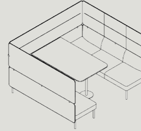
AHB6-S-2335-NA W 2335 D 2090 H 1350 S 440
