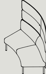
AHB45-D W 1660 D 1165 H 1350 S 440 IN Ø3300 / OUT Ø4760 W 65.4" D 45.9" H 53.1" S17.3" IN Ø129.9" / OUT Ø187.4"
