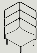
AHC1-D* W 730 D 730 H 1350 S 440 W 28.7" D 28.7" H 53.1" S17.3"
