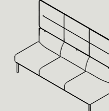
AHB3-S* W 2040 D 730 H 1350 S 440 W 80.3" D 28.7" H 53.1" S17.3"
