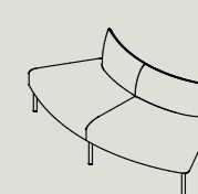
AB60-R W 1610 D 1315 H 700 S 440 IN Ø2300 / OUT Ø3760 W 63.4" D 51.8" H 27.6" S17.3" IN Ø90.6" / OUT Ø148.0"
