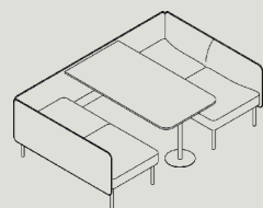
ALBT4-2185-NA W 2185 D 1410 H 700 S 440
