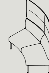
AHB45-S W 1660 D 1165 H 1350 S 440 IN Ø3300 / OUT Ø4760 W 65.4" D 45.9" H 53.1" S17.3" IN Ø129.9" / OUT Ø187.4"
