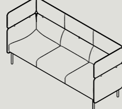
AML3 W 2140 D 730 H 1025 S 440 W 84.25" D 28.7" H 40.4" S17.3"
