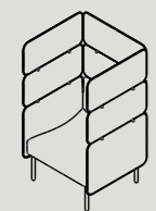
AHL1-D W 825 D 730 H 1350 S 440 W 32.5" D 28.7" H 53.1" S17.3"
