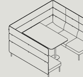
AHB6-D-2335-NA W 2335 D 2090 H 1350 S 440
