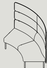
AHB60-D W 1660 D 1315 H 1350 S 440 IN Ø2400 / OUT Ø3,860 W 65.4" D 51.8" H 53.1" S17.3" IN Ø94.5" / OUT Ø152.0"
