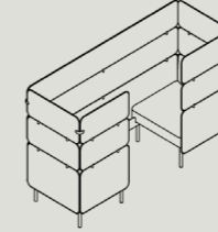
AHB2-D-2185-ARM W 2185 D 825 H 1350 S 440
