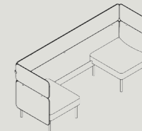
AMBT2-2335-NA W 2335 D 775 H 1025 S 440
