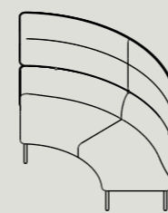
AHB90-S W 1530 D 1530 H 1350 S 440 IN Ø1600 / OUT Ø3,040 W 60.2" D 60.2" H 53.1" S17.3" IN Ø63.0" / OUT Ø119.7"
