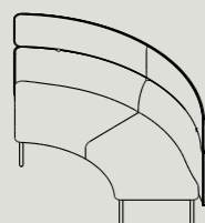
AMB90 W 1530 D 1530 H 1025 S 440 IN Ø1600 / OUT Ø3040 W 60.2" D 60.2" H 40.4" S17.3" IN Ø63.0" / OUT Ø119.7"
