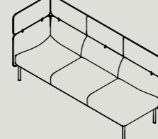
AMA3-R/L** W 2090 D 730 H 1025 S 440 W 82.3" D 28.7" H 40.4" S17.3"
