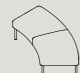
AO45 W 1610 D 1115 H 440 IN Ø3300 / OUT Ø4660 W 63.4" D 43.9" H 17.3" IN Ø129.9" / OUT Ø183.5"
