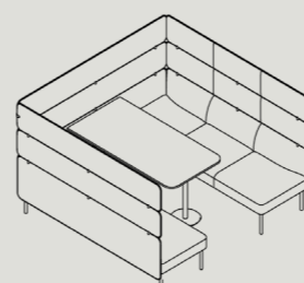
AHB6-D-2185-NA W 2185 D 2090 H 1350 S 440
