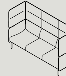
AHL3-S W 2140 D 730 H 1350 S 440 W 84.25" D 28.7" H 53.1" S17.3"
