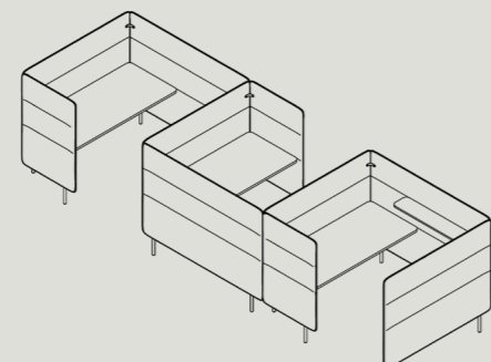
AWH-S-PL3-A-XXXX 1330 - W 5370 / D 1460 / H 1350 1520 - W 5370 / D 1650 / H 1350 1710 - W 5370 / D 1840 / H 1350
