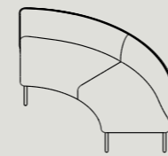
AB90 W 1530 D 1530 H 700 S 440 IN Ø1600 / OUT Ø3040 W 60.2" D 60.2" H 27.6" S17.3" IN Ø63.0" / OUT Ø119.7"
