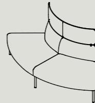
AMB90-R W 1480 D 1480 H 1025 S 440 IN Ø1500 / OUT Ø2960 W 58.3" D 58.3" H 40.4" S17.3" IN Ø59.1" / OUT Ø116.5"
