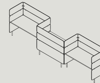
AWH-D-OL3-A-XXXX 1330 - W 4250 / D 825 / H 1350 1520 - W 4820 / D 825 / H 1350 1710 - W 5390 / D 825 / H 1350
