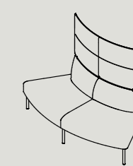
AHB60-R-S W 1610 D 1315 H 1350 S 440 IN Ø2300 / OUT Ø3,760 W 63.4" D 51.8" H 53.1" S17.3" IN Ø90.6" / OUT Ø148.0"
