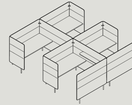
AWH-S-PL4-B-XXXX W 3605 / D 2855 / H 1350 W 3605 / D 3235 / H 1350 W 3605 / D 3615 / H 1350
