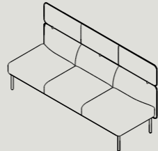
AMB3* W 2040 D 730 H 1025 S 440 W 80.3" D 28.7" H 40.4" S17.3"
