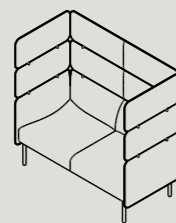
AHL2-D W 1460 D 730 H 1350 S 440 W 57.5" D 28.7" H 53.1" S17.3"
