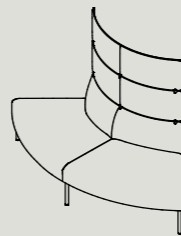
AHB90-R-D W 1480 D 1480 H 1350 S 440 IN Ø1500 / OUT Ø2,960 W 58.3" D 58.3" H 53.1" S17.3" IN Ø59.1" / OUT Ø116.5"
