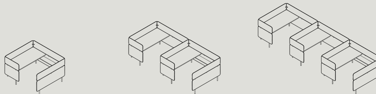
AWM-PL1-XXXX 1330 - W 1840 / D 1460 / H 1025 1520 - W 1840 / D 1650 / H 1025 1710 - W 1840 / D 1840 / H 1025
