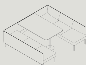
ALBT6-2335-NA W 2335 D 2090 H 700 S 440
