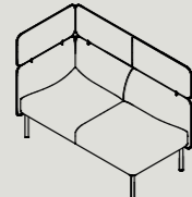
AMA2-R/L** W 1410 D 730 H 1025 S 440 W 55.5" D 28.7" H 40.4" S17.3"
