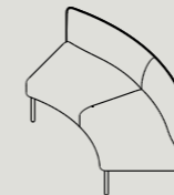
AB60 W 1660 D 1315 H 700 S 440 IN Ø2400 / OUT Ø3860 W 65.4" D 51.8" H 27.6" S17.3" IN Ø94.5" / OUT Ø152.0"
