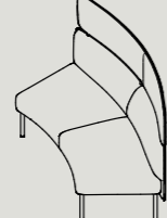
AMB45 W 1660 D 1165 H 1025 S 440 IN Ø3300 / OUT Ø4760 W 65.4" D 45.9" H 40.4" S17.3" IN Ø129.9" / OUT Ø187.4"
