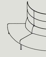
AHB90-R-S W 1480 D 1480 H 1350 S 440 IN Ø1500 / OUT Ø2,960 W 58.3" D 58.3" H 53.1" S17.3" IN Ø59.1" / OUT Ø116.5"
