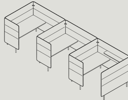
AWH-S-PL3-XXXX 1330 - W 5370 / D 1460 / H 1350 1520 - W 5370 / D 1650 / H 1350 1710 - W 5370 / D 1840 / H 1350
