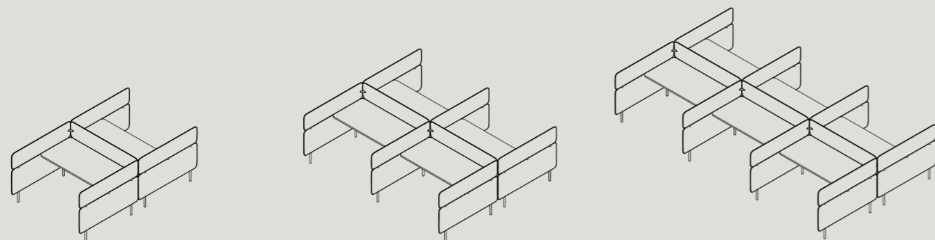
AWM-SPL2-B-XXXX 1330 - W 1460 / D 2845 / H 1025 1520 - W 1650 / D 2845 / H 1025 1710 - W 1840 / D 2845 / H 1025
