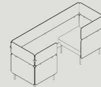
AMBT2-2185-ARM W 2185 D 825 H 1025 S 440
