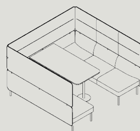
AHB6-S-2185-NA W 2185 D 2090 H 1350 S 440
