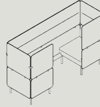
AHB2-S-2335-ARM W 2335 D 825 H 1350 S 440
