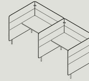
AWH-S-SPL2-XXXX 1330 - W 2855 / D 1460 / H 1350 1520 - W 3235 / D 1460 / H 1350 1710 - W 3615 / D 1460 / H 1350
