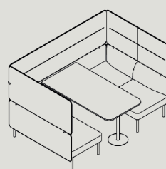
AHB4-S-2185-NA W 2185 D 1410 H 1350 S 440
