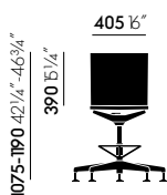
.04 Counter (glides)
