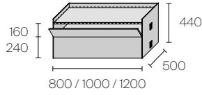
Suspended unit with flap door high side
