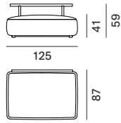
module seat M with back structure L110
