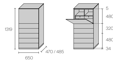
Self
