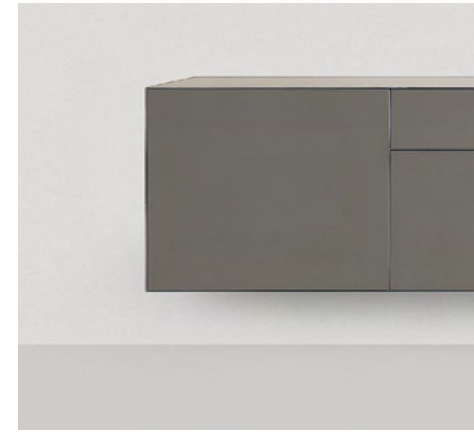
Suspended composition
